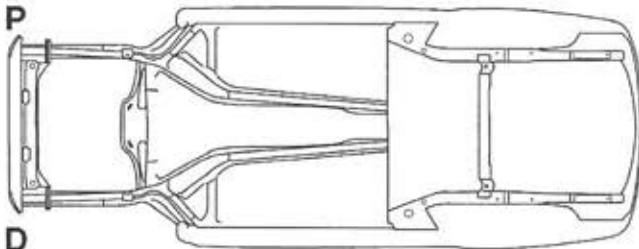
UNDERBODY VIEW
